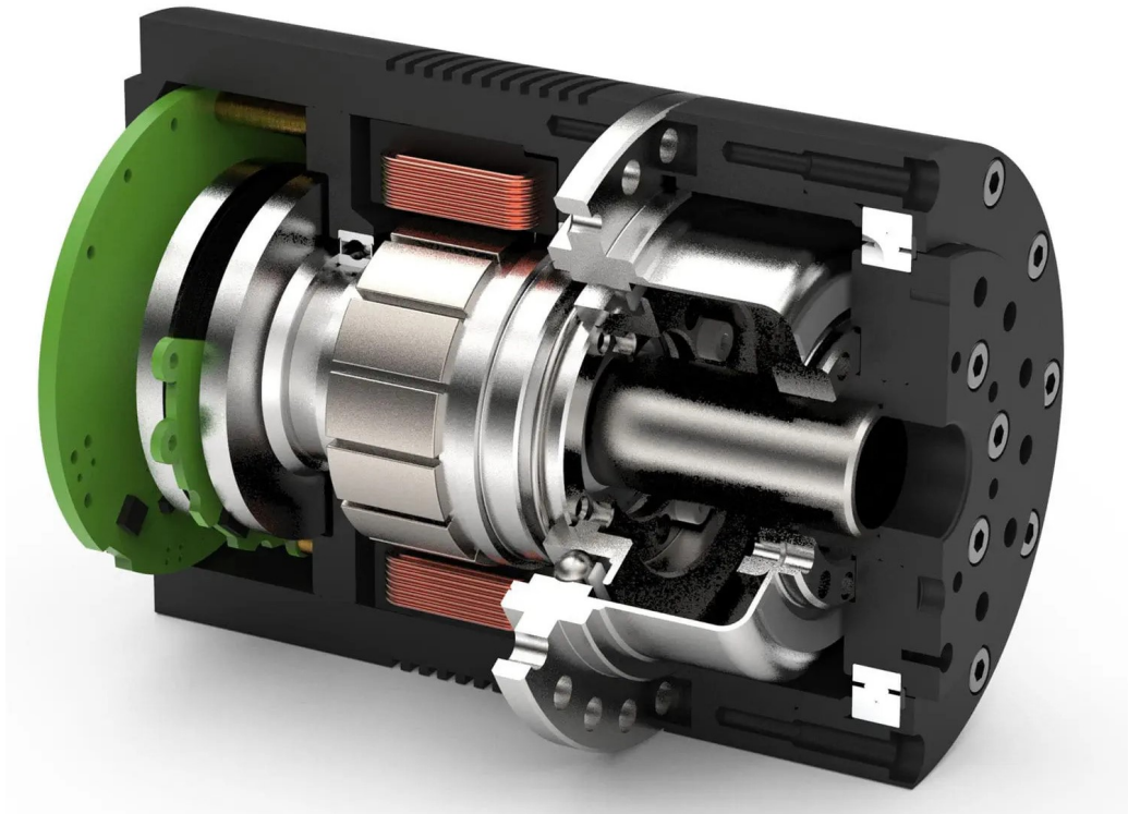
Figure 1: Rdrive motor by Rozum® www.rozum.com
